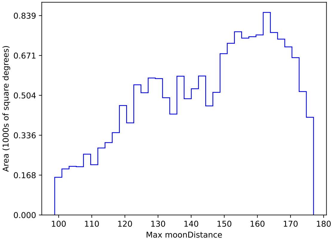
too_elab_r16_d2_giz_v3.4_10yrs WFD y band: Max moonDistance
