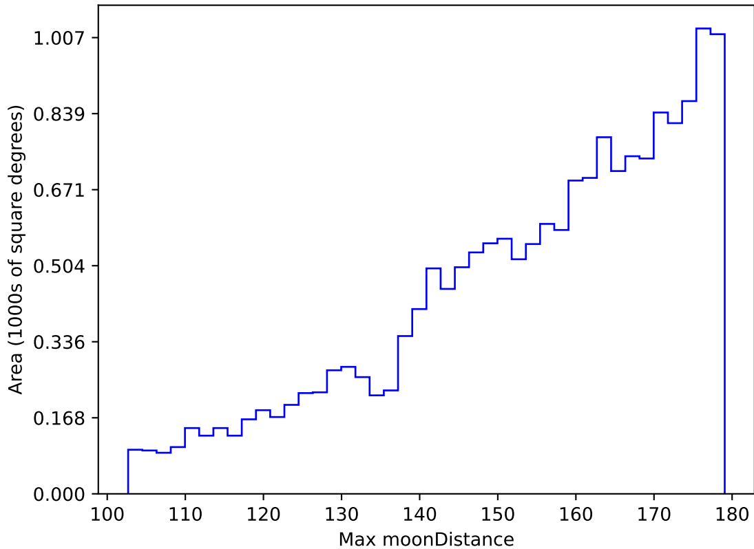
too_elab_r16_d2_giz_v3.4_10yrs WFD u band: Max moonDistance
