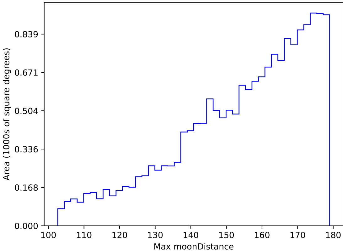
too_elab_r16_d2_giz_v3.4_10yrs WFD g band: Max moonDistance
