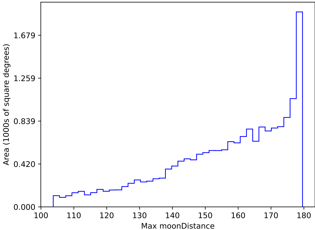
too_elab_r16_d2_giz_v3.4_10yrs WFD all bands: Max moonDistance
