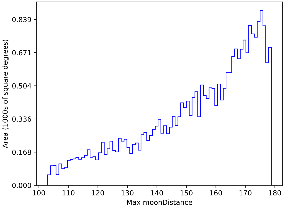
too_elab_r16_d2_giz_v3.4_10yrs All sky z band: Max moonDistance
