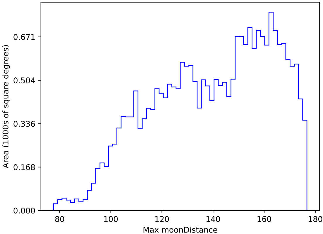
too_elab_r16_d2_giz_v3.4_10yrs All sky y band: Max moonDistance
