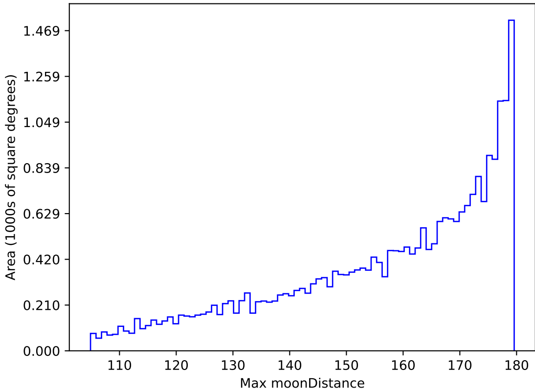
too_elab_r16_d2_giz_v3.4_10yrs All sky all bands: Max moonDistance
