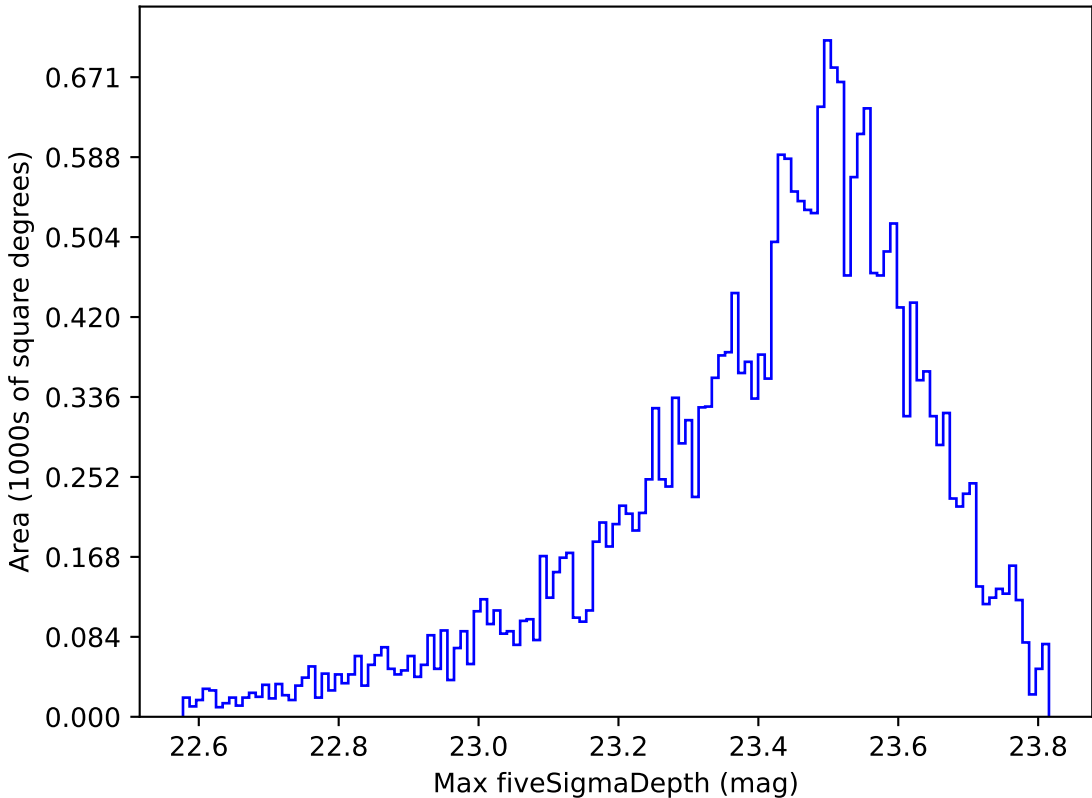
too_elab_r16_d2_giz_v3.4_10yrs Yr 1 z band: Max fiveSigmaDepth
