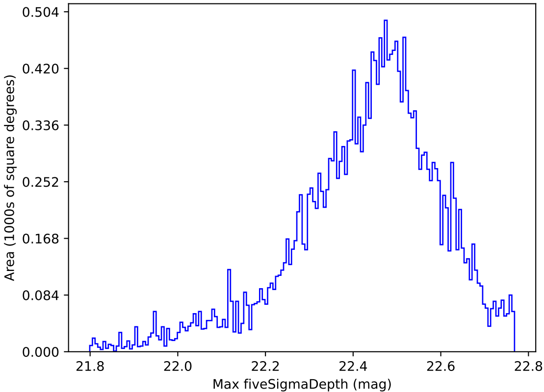
too_elab_r16_d2_giz_v3.4_10yrs Yr 1 y band: Max fiveSigmaDepth
