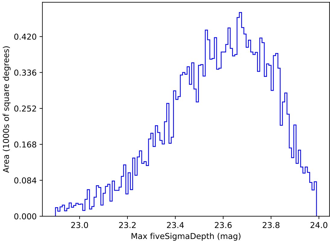
too_elab_r16_d2_giz_v3.4_10yrs Yr 1 u band: Max fiveSigmaDepth
