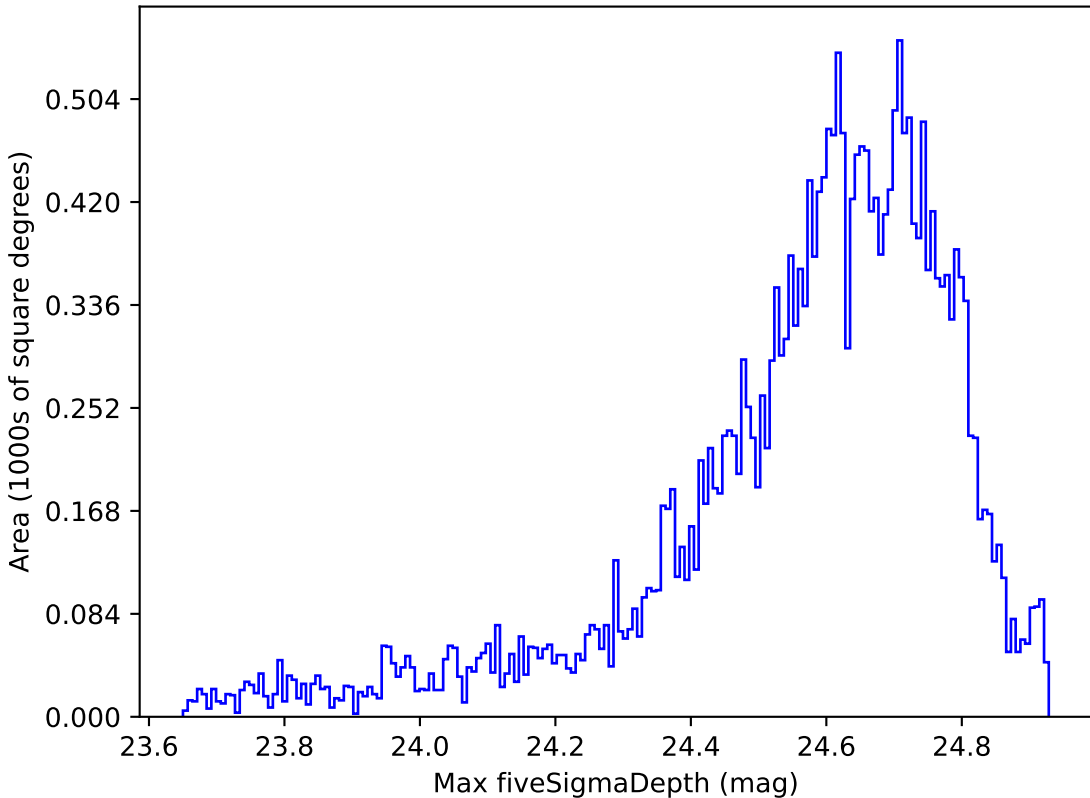
too_elab_r16_d2_giz_v3.4_10yrs Yr 1 r band: Max fiveSigmaDepth
