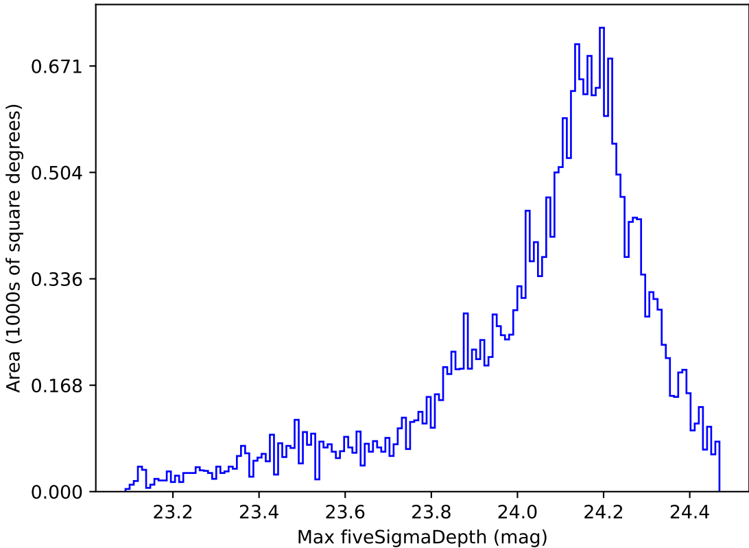
too_elab_r16_d2_giz_v3.4_10yrs Yr 1 i band: Max fiveSigmaDepth
