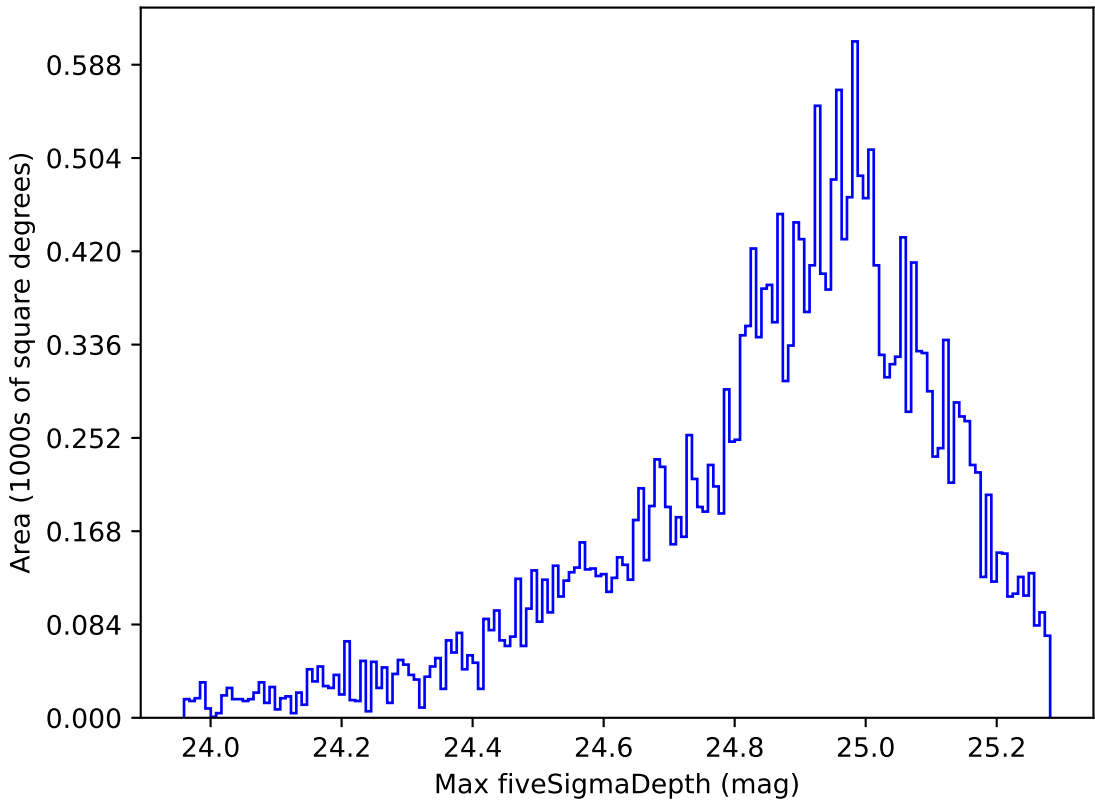
too_elab_r16_d2_giz_v3.4_10yrs Yr 1 g band: Max fiveSigmaDepth
