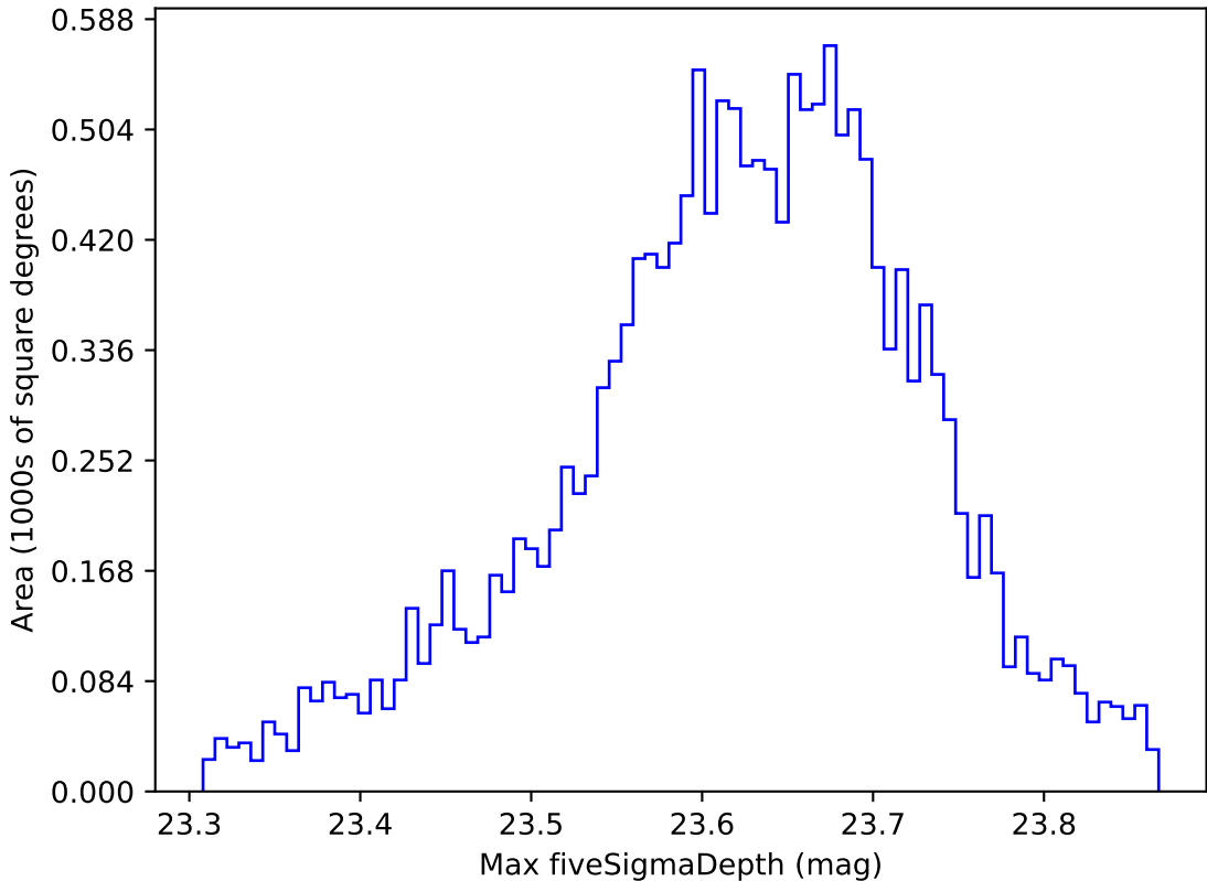
too_elab_r16_d2_giz_v3.4_10yrs WFD z band: Max fiveSigmaDepth
