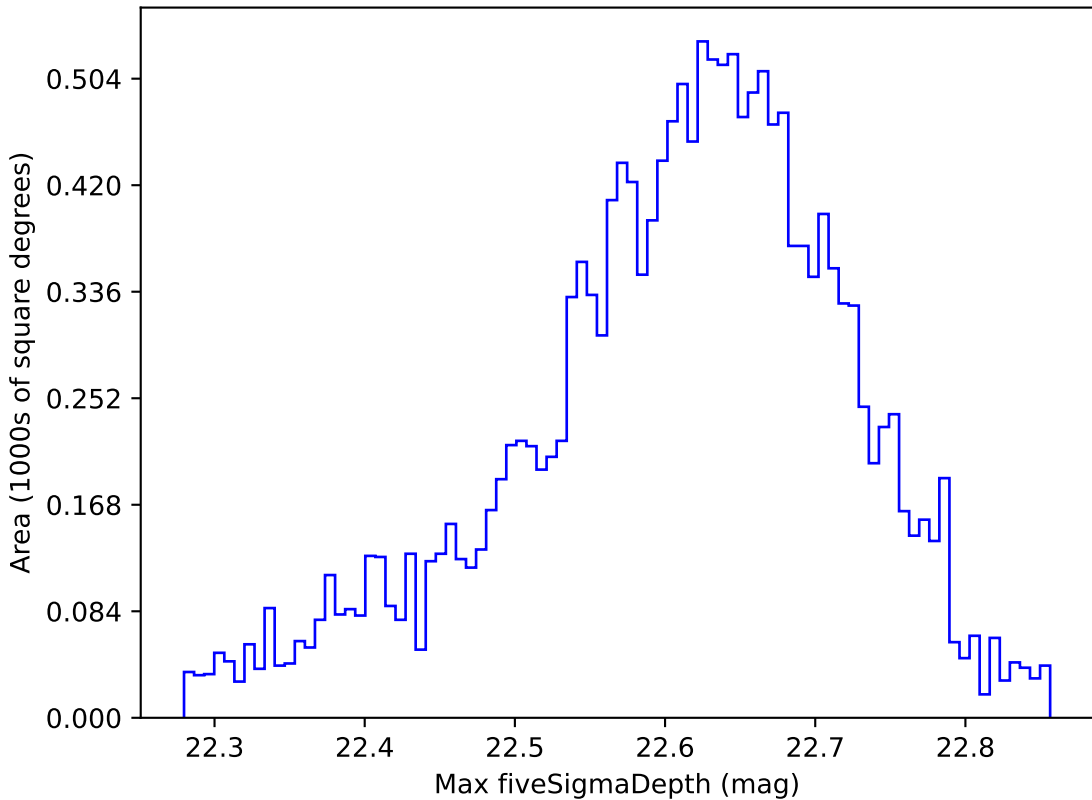
too_elab_r16_d2_giz_v3.4_10yrs WFD y band: Max fiveSigmaDepth
