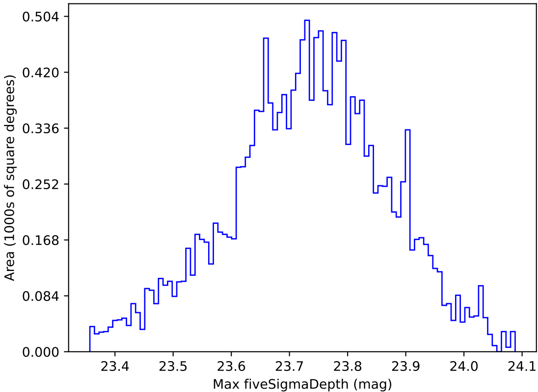
too_elab_r16_d2_giz_v3.4_10yrs WFD u band: Max fiveSigmaDepth
