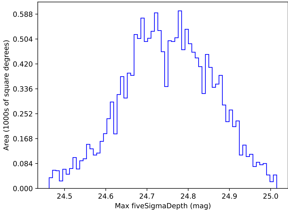
too_elab_r16_d2_giz_v3.4_10yrs WFD r band: Max fiveSigmaDepth
