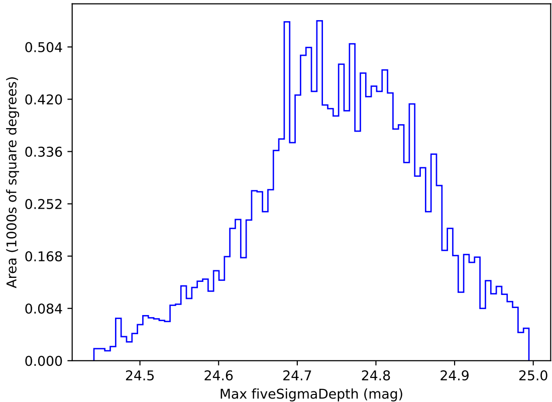
too_elab_r16_d2_giz_v3.4_10yrs WFD r band: Max fiveSigmaDepth
