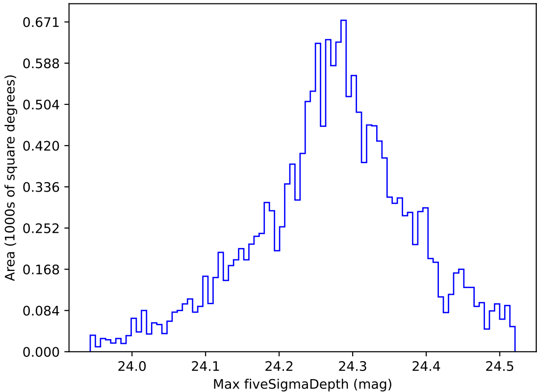
too_elab_r16_d2_giz_v3.4_10yrs WFD i band: Max fiveSigmaDepth
