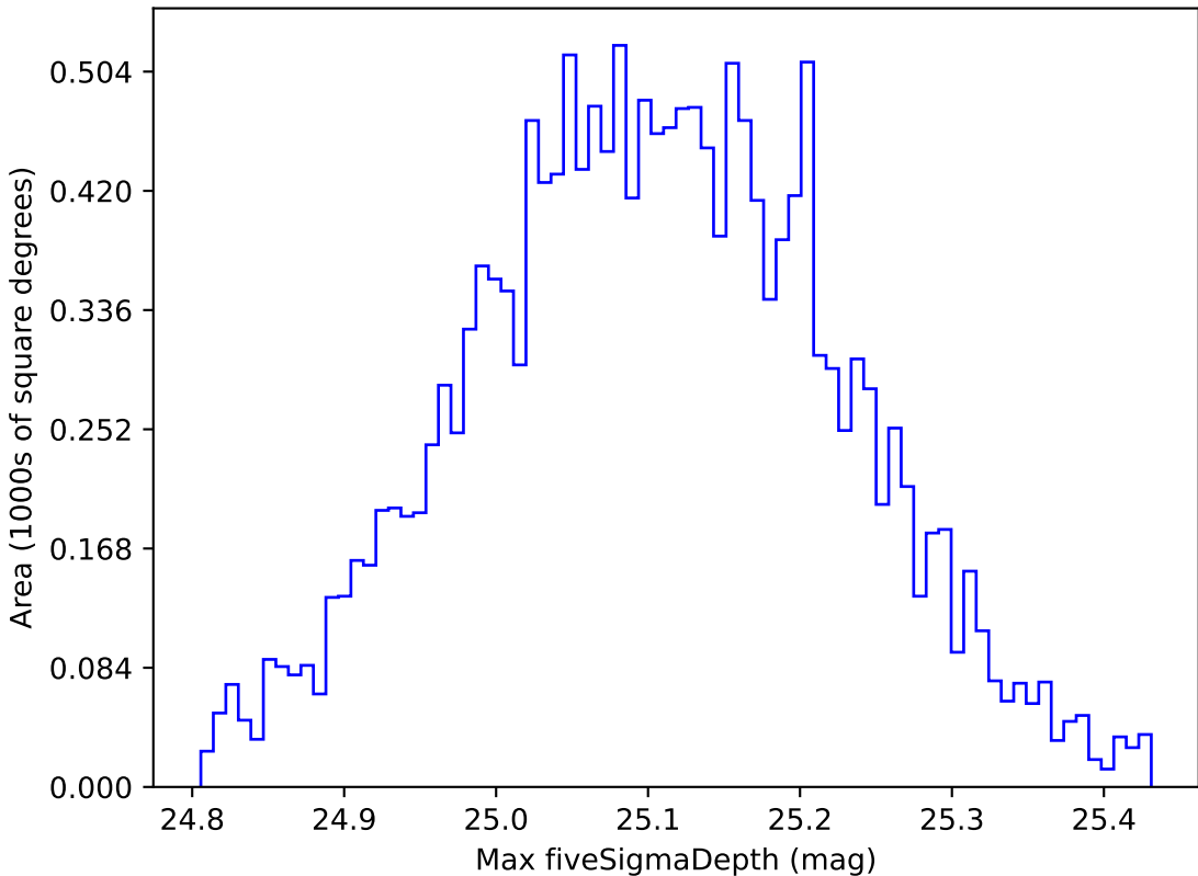
too_elab_r16_d2_giz_v3.4_10yrs WFD g band: Max fiveSigmaDepth
