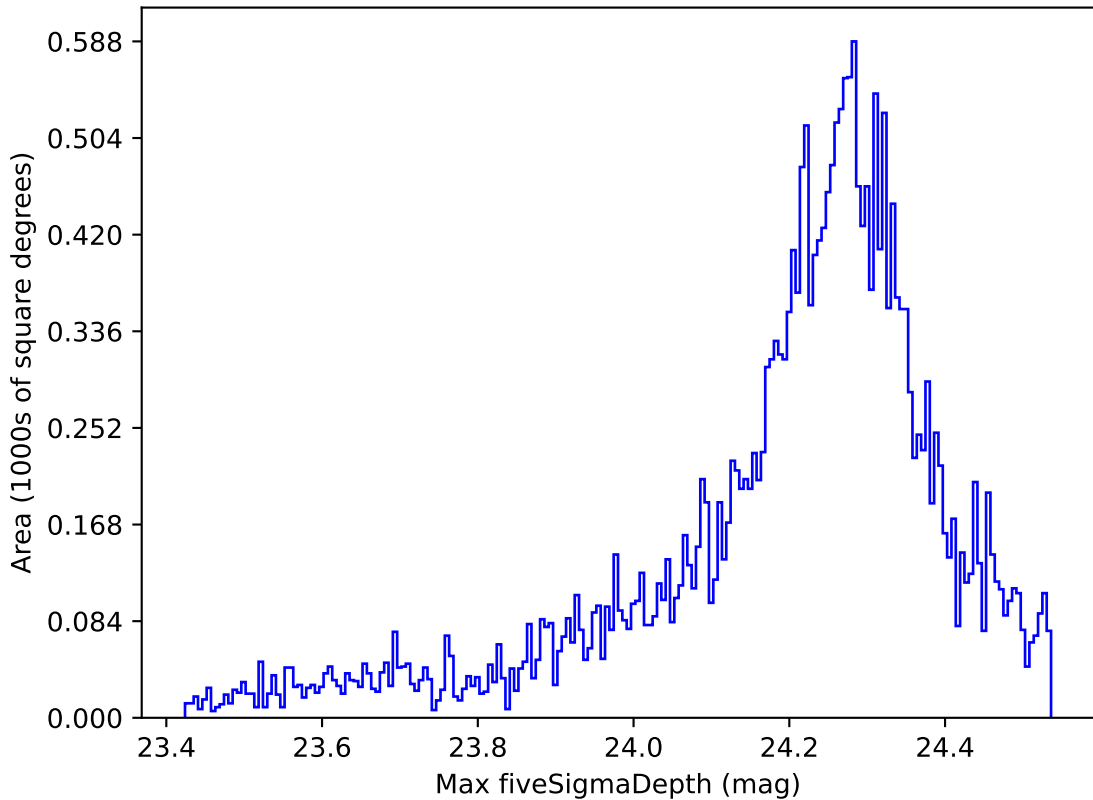
too_elab_r16_d2_giz_v3.4_10yrs All sky i band: Max fiveSigmaDepth
