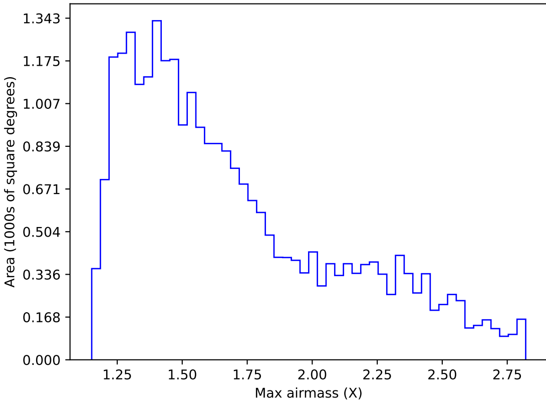
too_elab_r16_d2_giz_v3.4_10yrs Yr 1 z band: Max airmass
