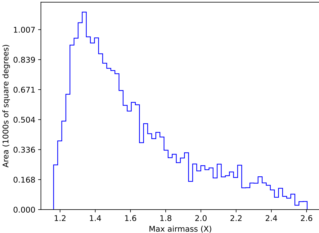
too_elab_r16_d2_giz_v3.4_10yrs Yr 1 y band: Max airmass
