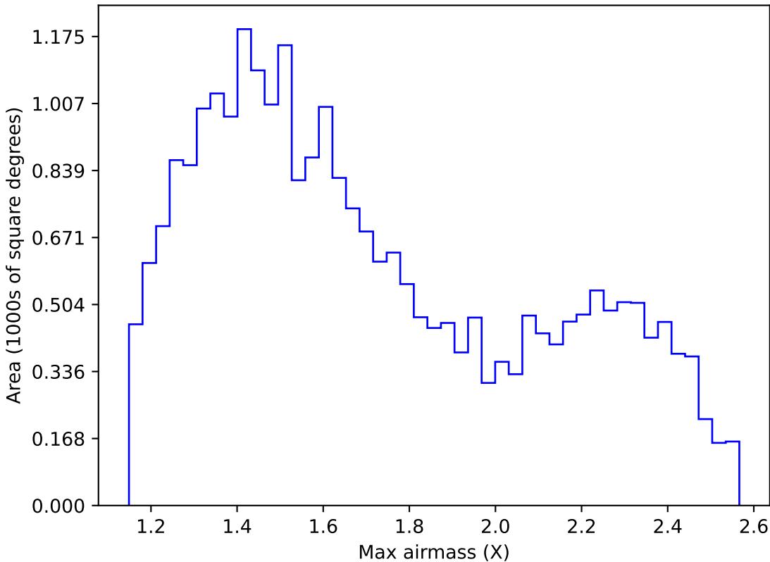
too_elab_r16_d2_giz_v3.4_10yrs Yr 1 r band: Max airmass
