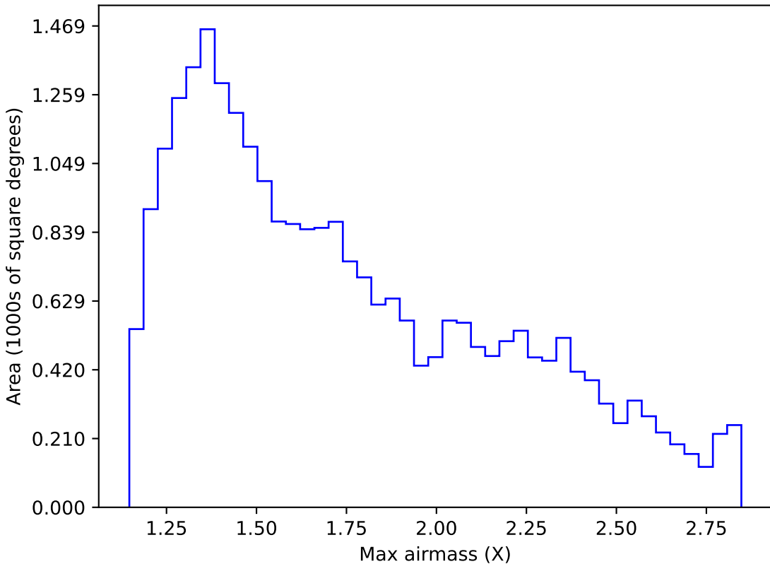
too_elab_r16_d2_giz_v3.4_10yrs Yr 1 i band: Max airmass
