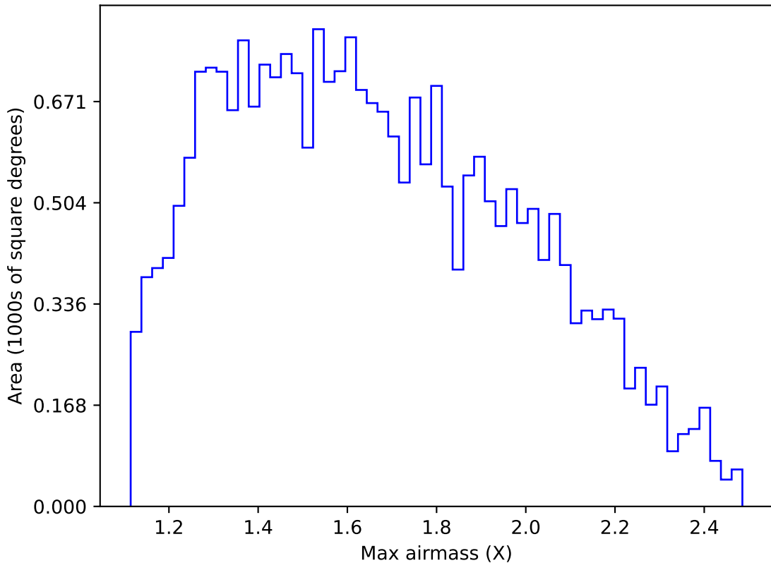
too_elab_r16_d2_giz_v3.4_10yrs Yr 1 g band: Max airmass
