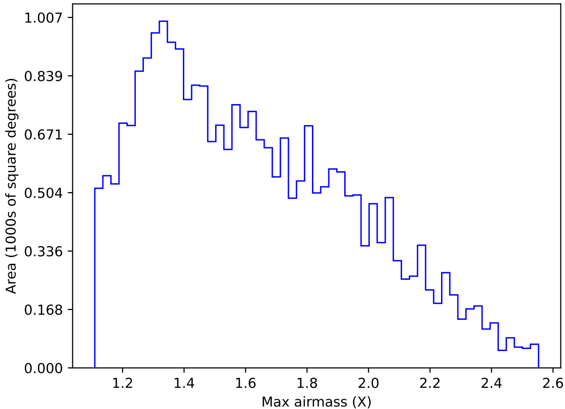
too_elab_r16_d2_giz_v3.4_10yrs Yr 1 g band: Max airmass
