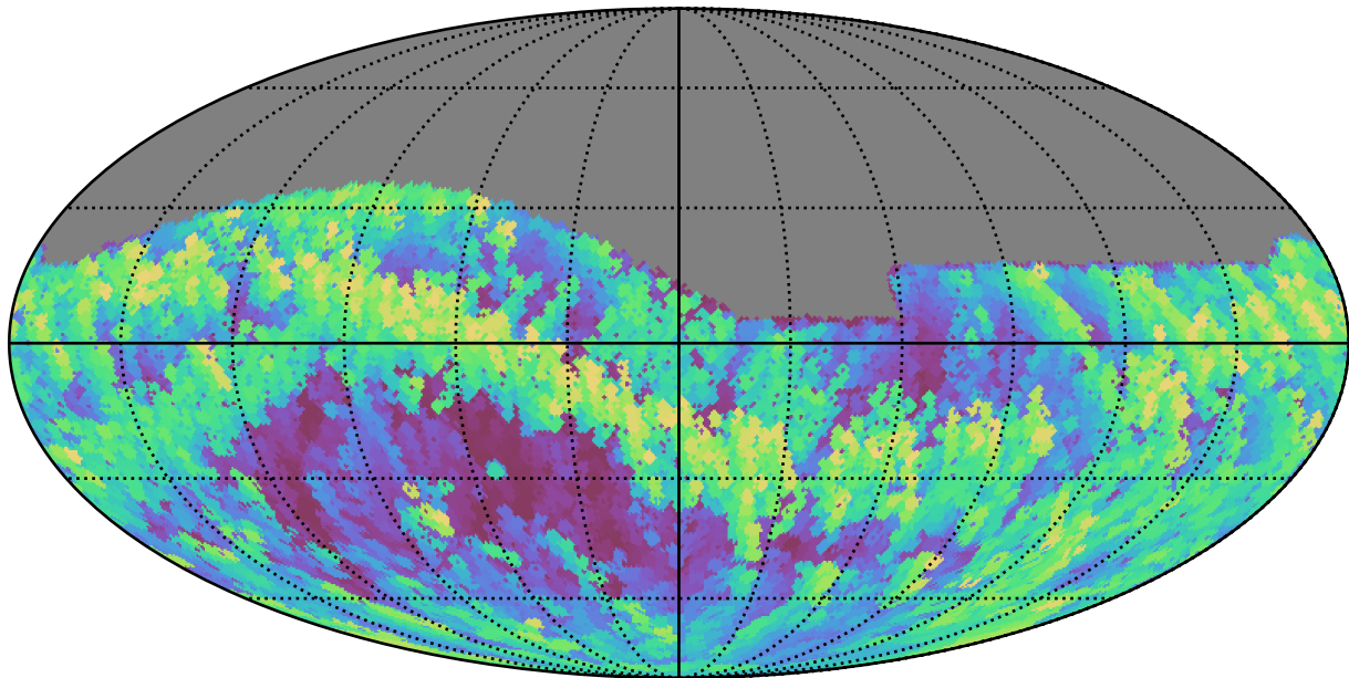
too_elab_r16_d2_giz_v3.4_10yrs Yr 1 all bands: Max airmass
