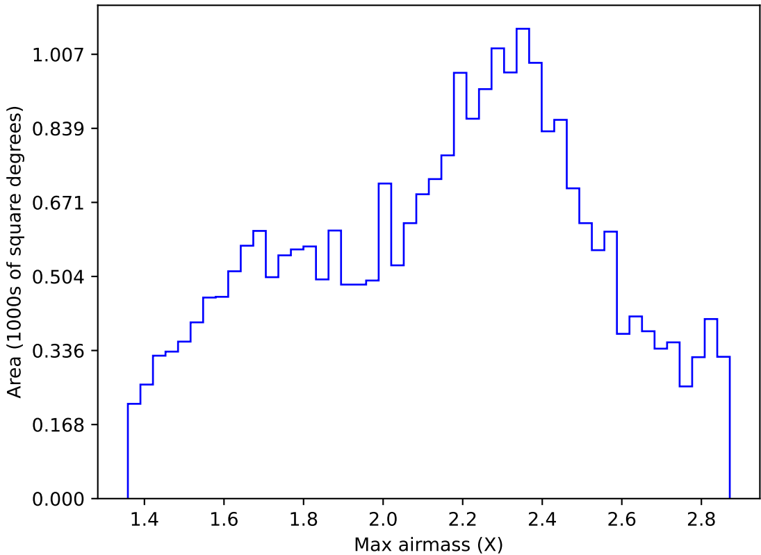
too_elab_r16_d2_giz_v3.4_10yrs Yr 1 all bands: Max airmass
