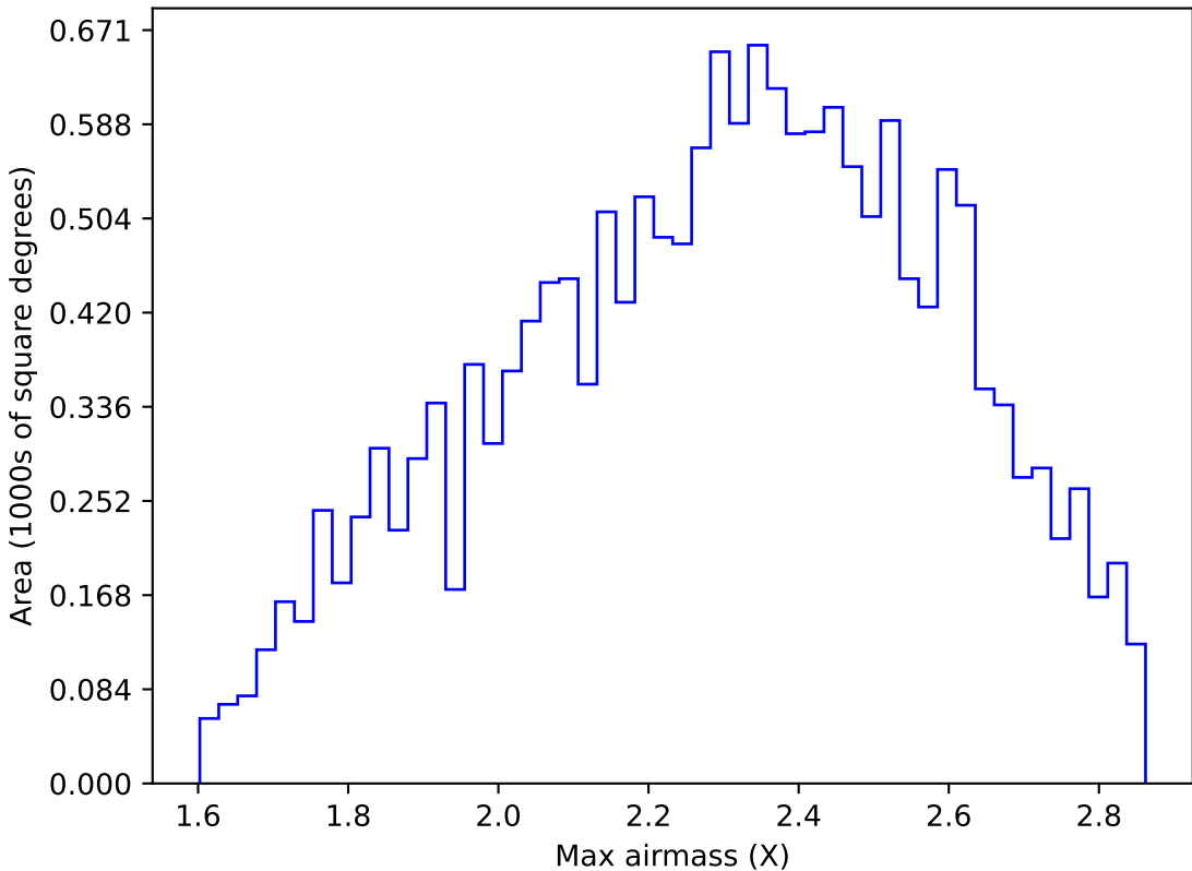
too_elab_r16_d2_giz_v3.4_10yrs WFD y band: Max airmass
