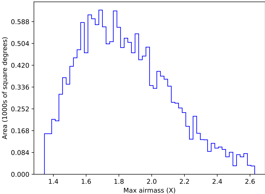
too_elab_r16_d2_giz_v3.4_10yrs WFD u band: Max airmass
