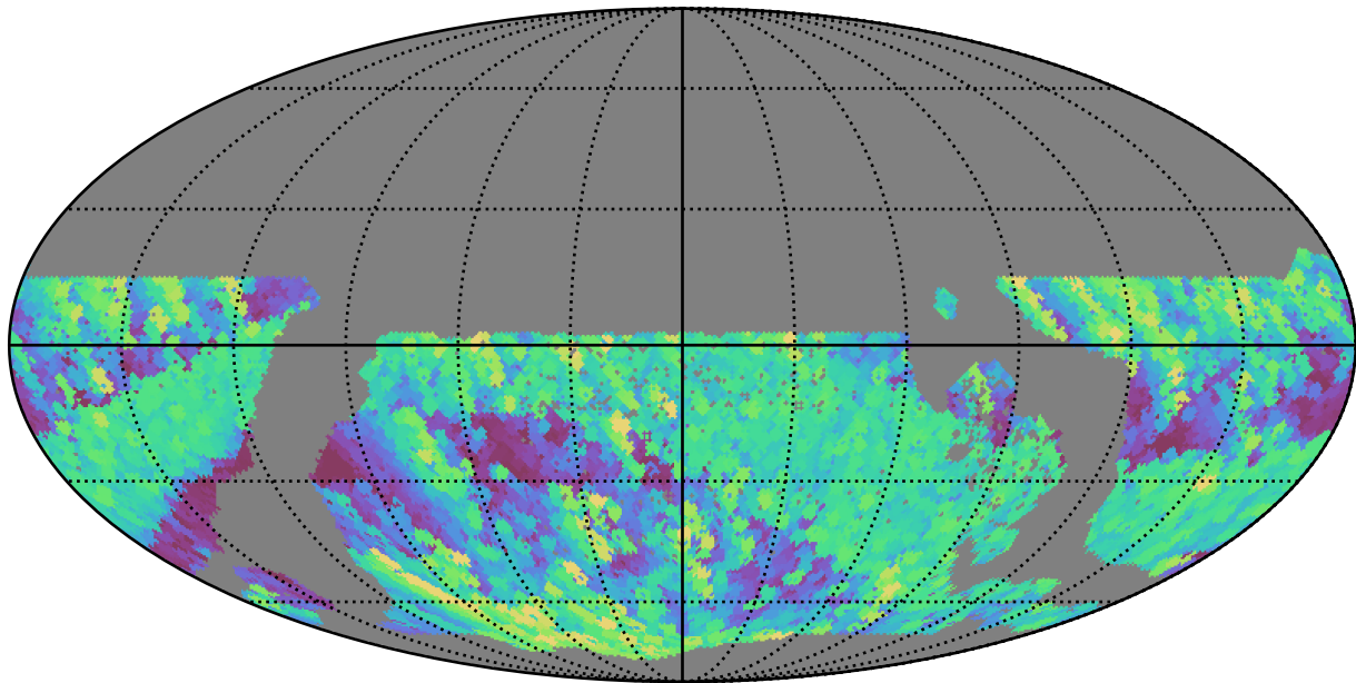
too_elab_r16_d2_giz_v3.4_10yrs WFD r band: Max airmass
