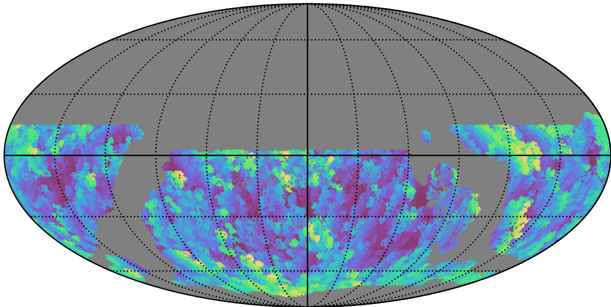
too_elab_r16_d2_giz_v3.4_10yrs WFD g band: Max airmass
