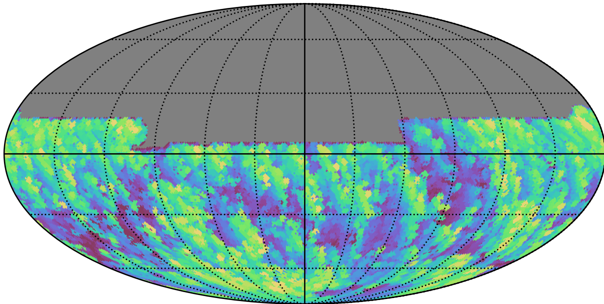
too_elab_r16_d2_giz_v3.4_10yrs All sky y band: Max airmass
