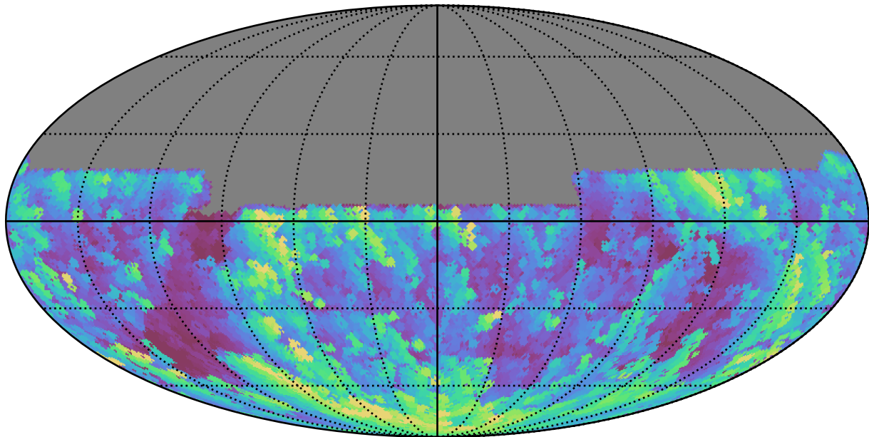
too_elab_r16_d2_giz_v3.4_10yrs All sky u band: Max airmass
