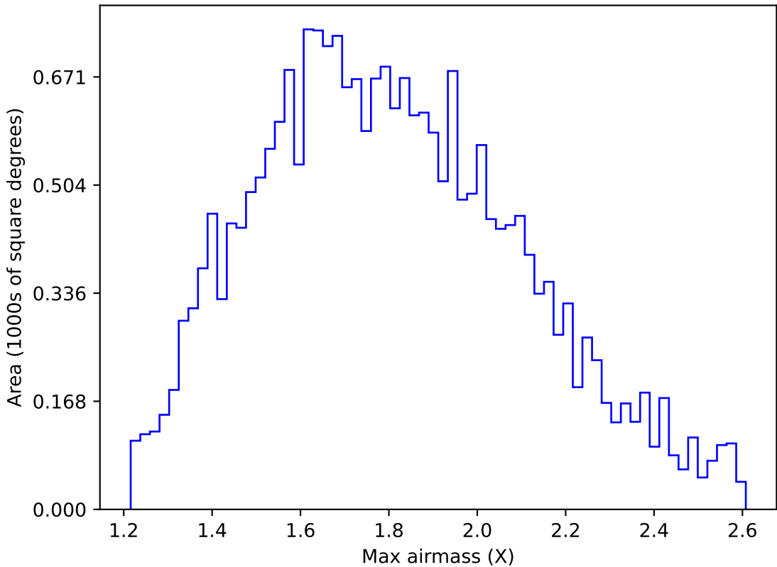
too_elab_r16_d2_giz_v3.4_10yrs All sky u band: Max airmass
