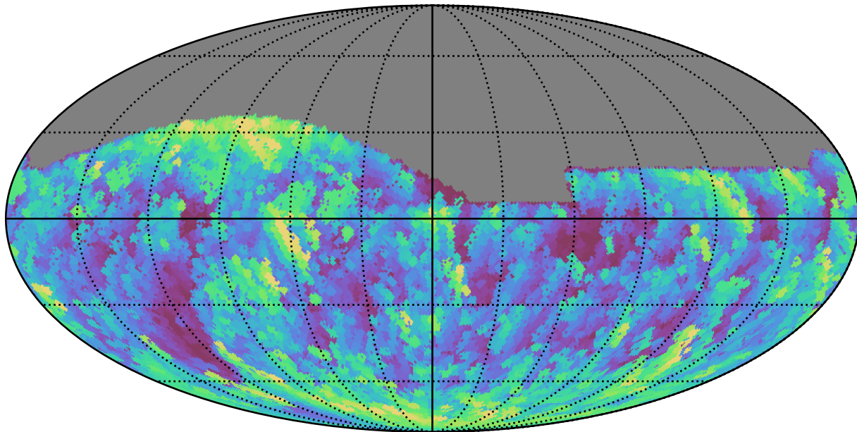
too_elab_r16_d2_giz_v3.4_10yrs All sky g band: Max airmass
