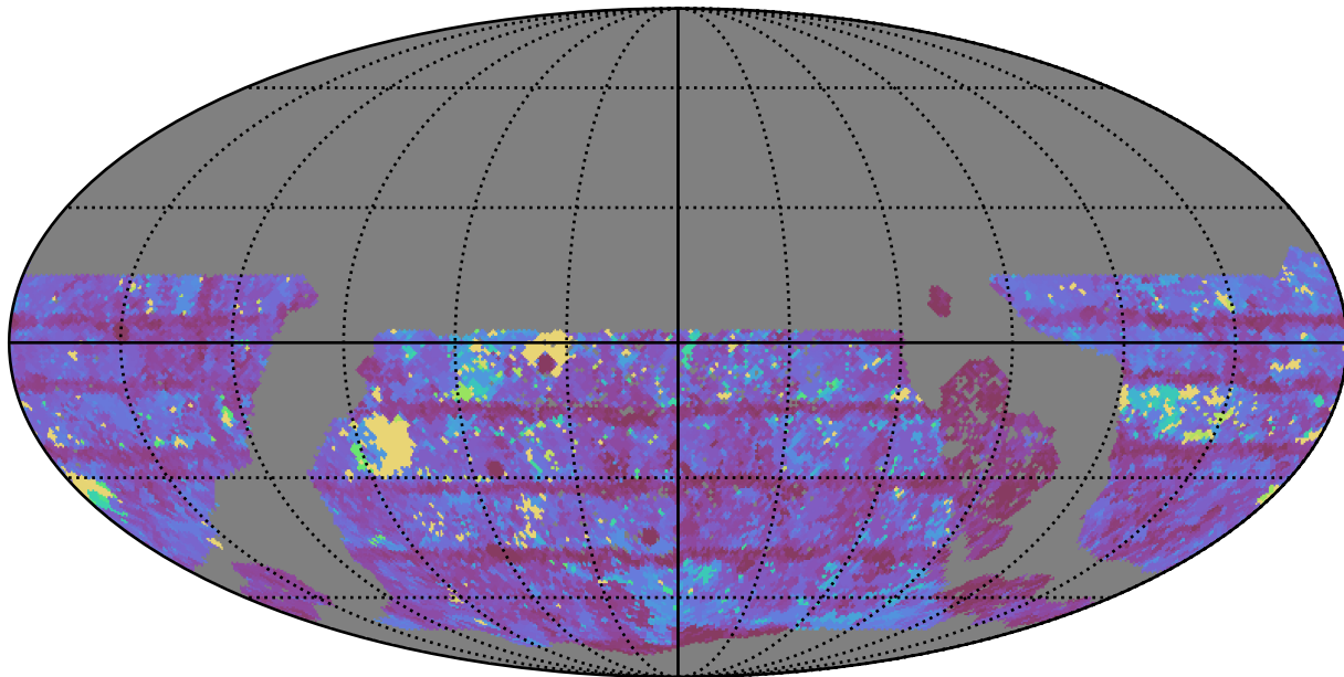
too_elab_r16_d2_giz_v3.4_10yrs WFD z band: Max Inter-Night Gap
