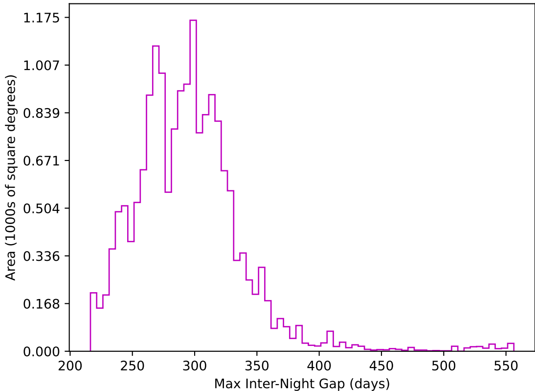
too_elab_r16_d2_giz_v3.4_10yrs WFD z band: Max Inter-Night Gap
