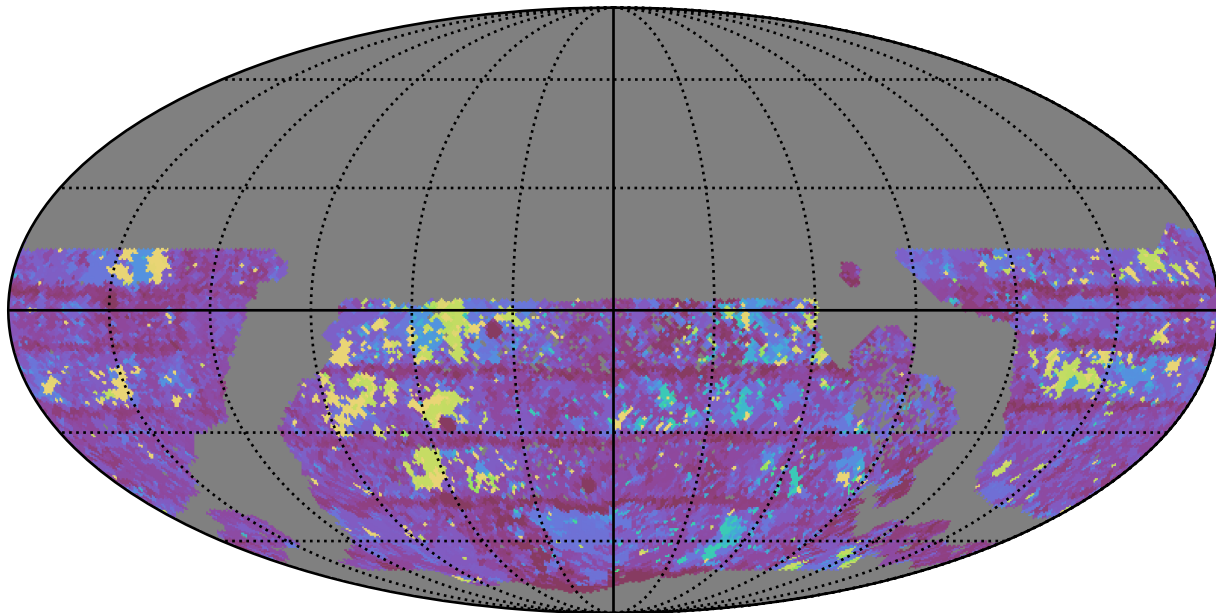
too_elab_r16_d2_giz_v3.4_10yrs WFD y band: Max Inter-Night Gap
