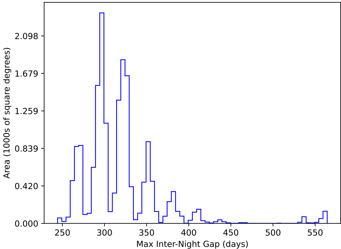
too_elab_r16_d2_giz_v3.4_10yrs WFD y band: Max Inter-Night Gap
