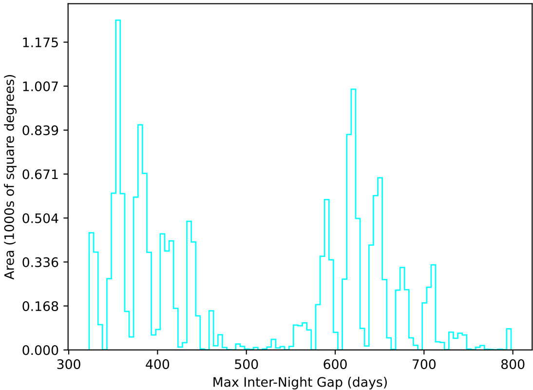
too_elab_r16_d2_giz_v3.4_10yrs WFD u band: Max Inter-Night Gap
