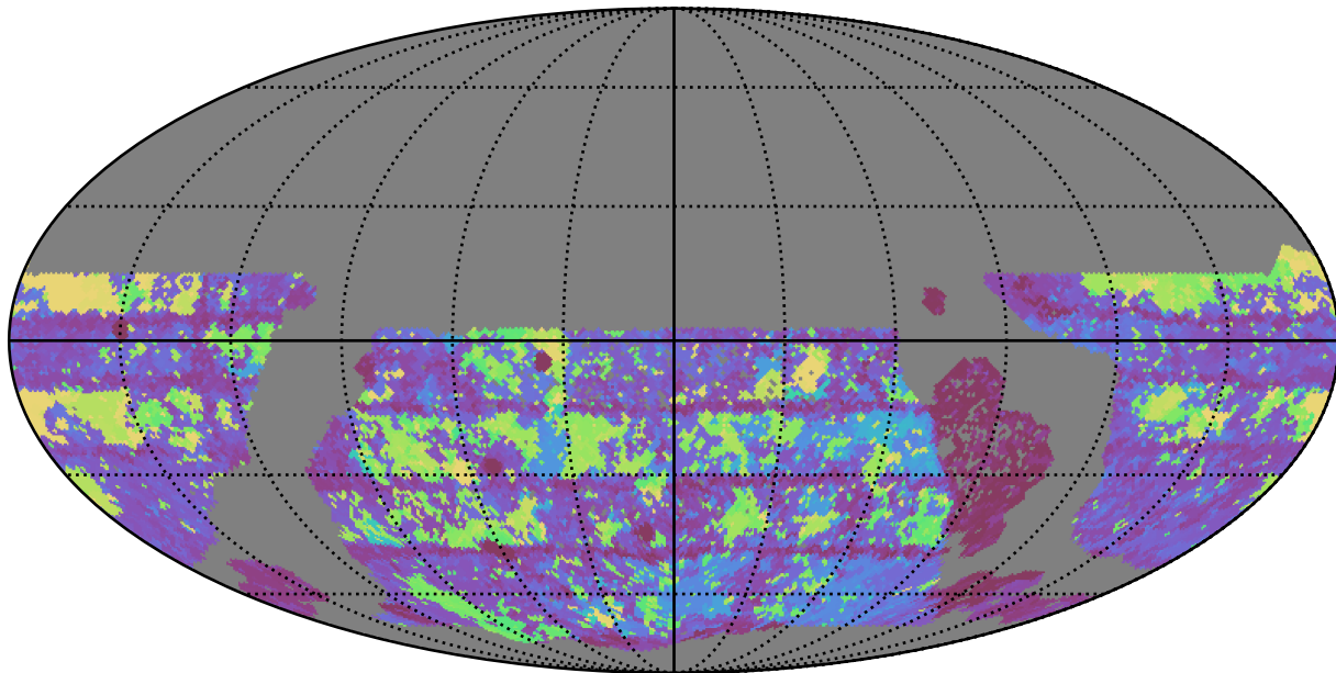
too_elab_r16_d2_giz_v3.4_10yrs WFD g band: Max Inter-Night Gap
