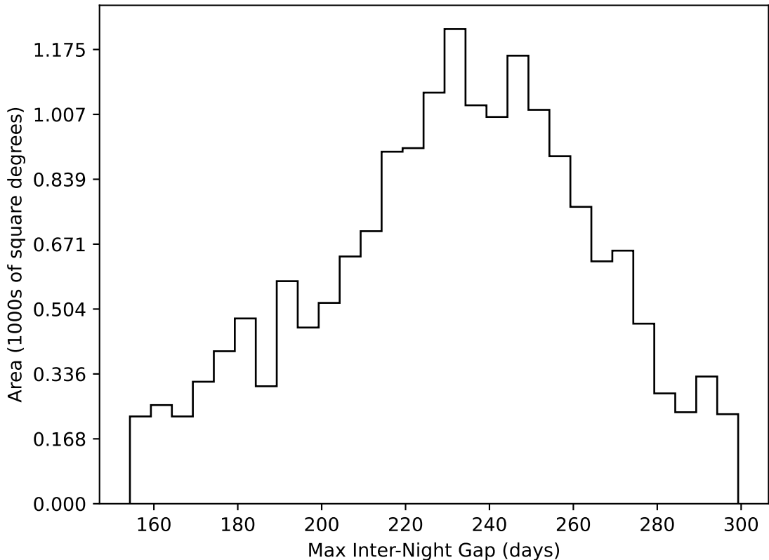
too_elab_r16_d2_giz_v3.4_10yrs WFD all bands: Max Inter-Night Gap
