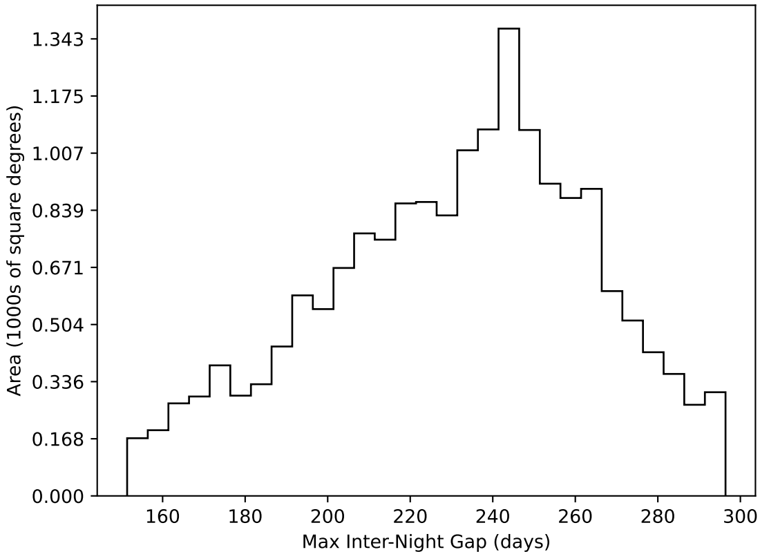
too_elab_r16_d2_giz_v3.4_10yrs WFD all bands: Max Inter-Night Gap
