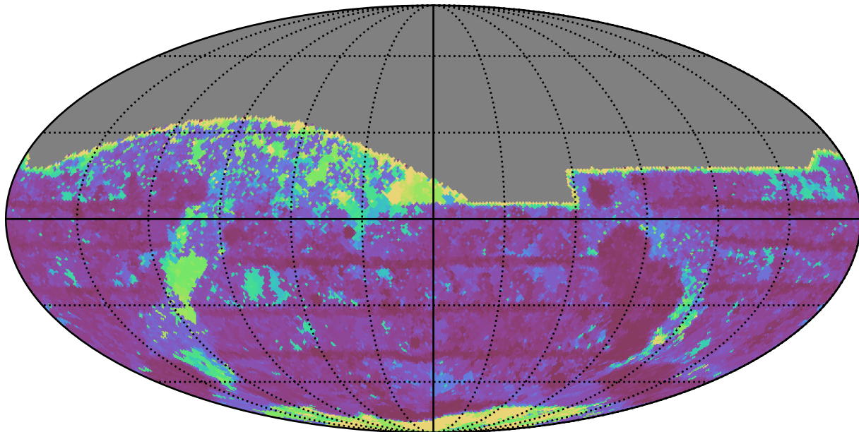
too_elab_r16_d2_giz_v3.4_10yrs All sky z band: Max Inter-Night Gap
