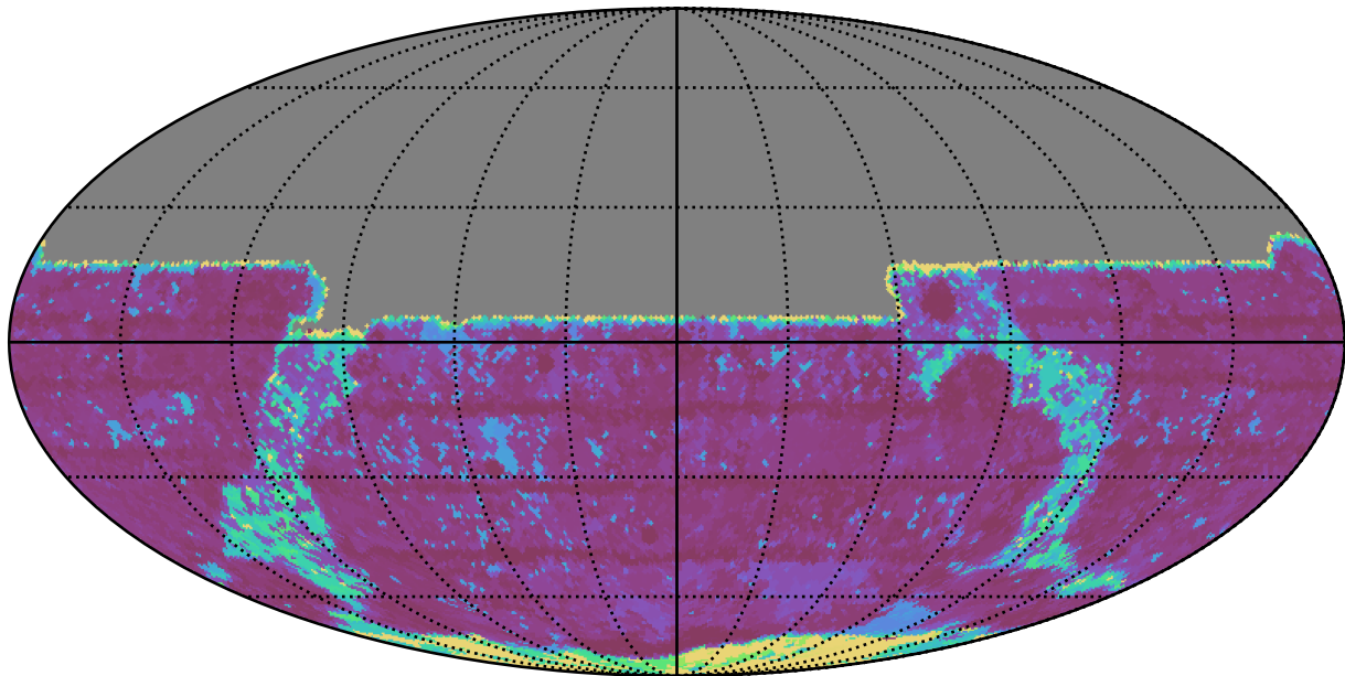
too_elab_r16_d2_giz_v3.4_10yrs All sky y band: Max Inter-Night Gap
