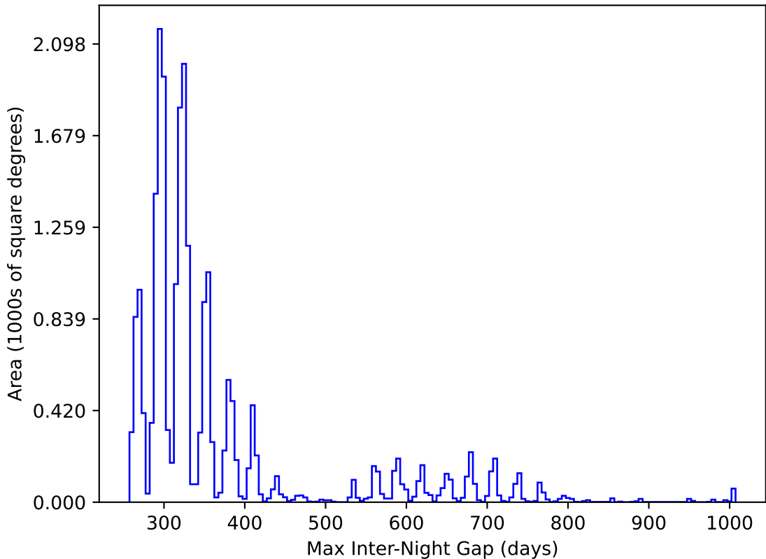
too_elab_r16_d2_giz_v3.4_10yrs All sky y band: Max Inter-Night Gap
