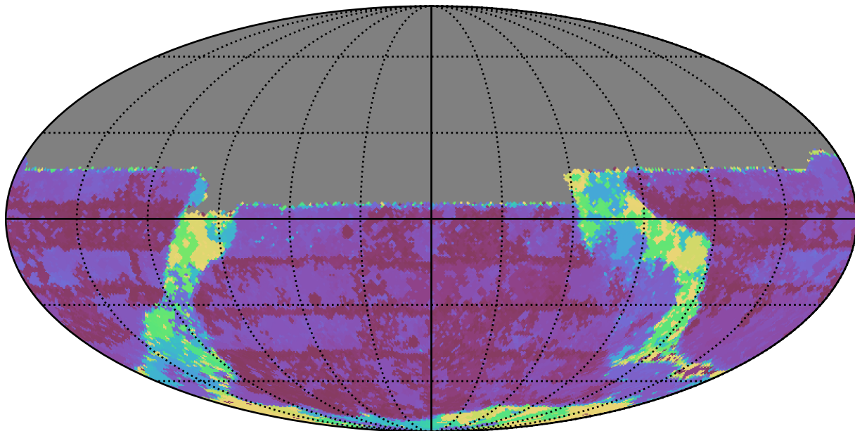
too_elab_r16_d2_giz_v3.4_10yrs All sky u band: Max Inter-Night Gap
