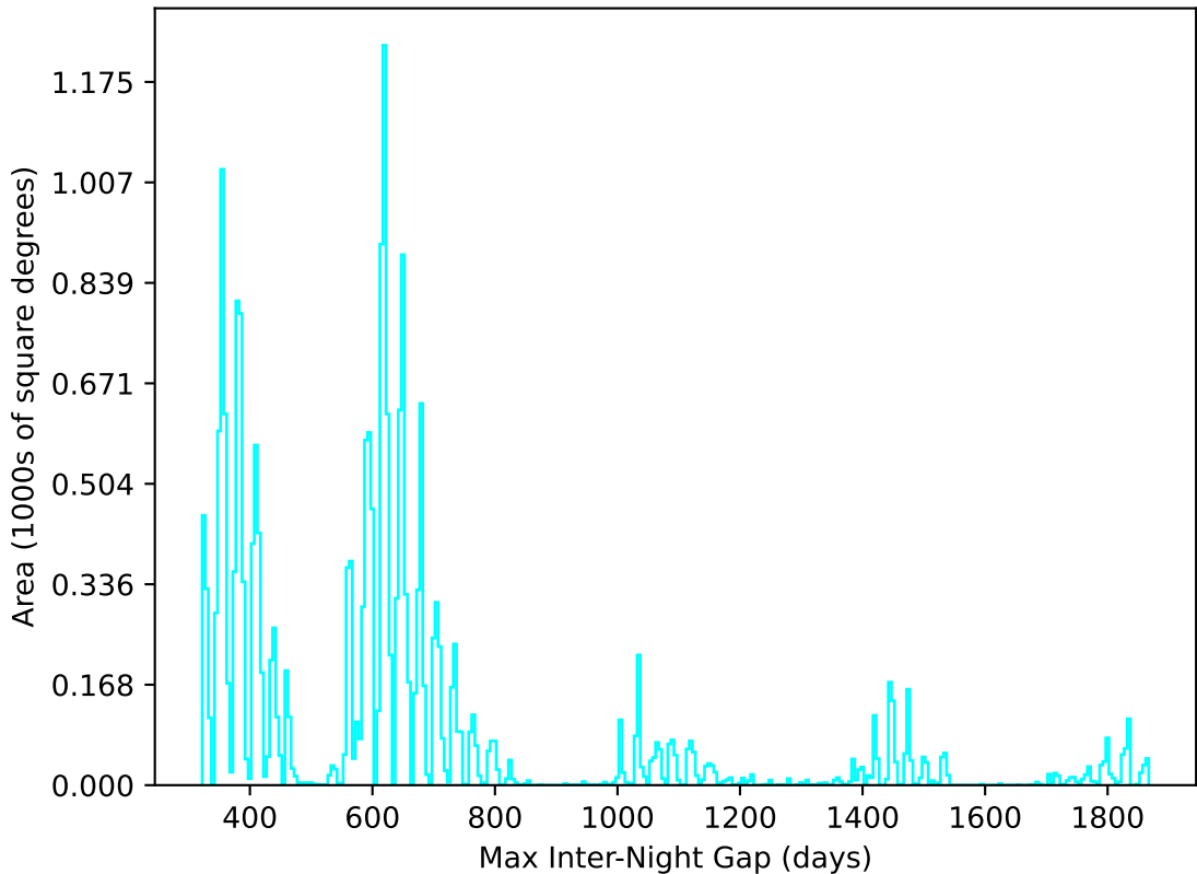
too_elab_r16_d2_giz_v3.4_10yrs All sky u band: Max Inter-Night Gap
