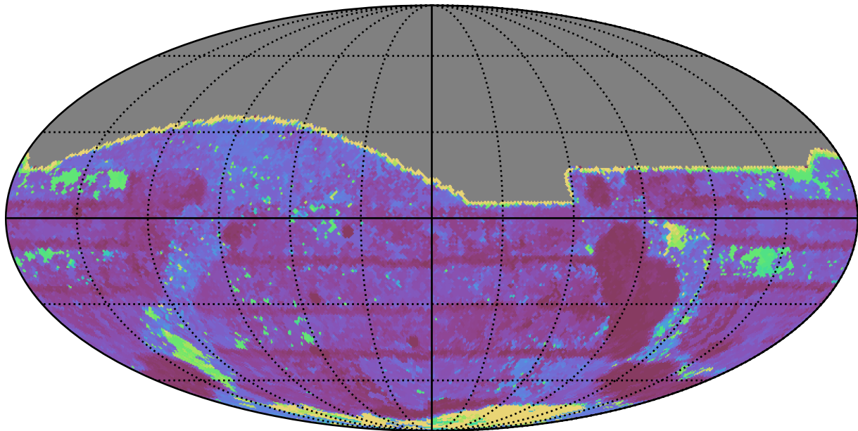
too_elab_r16_d2_giz_v3.4_10yrs All sky r band: Max Inter-Night Gap
