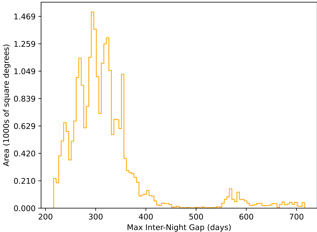
too_elab_r16_d2_giz_v3.4_10yrs All sky r band: Max Inter-Night Gap
