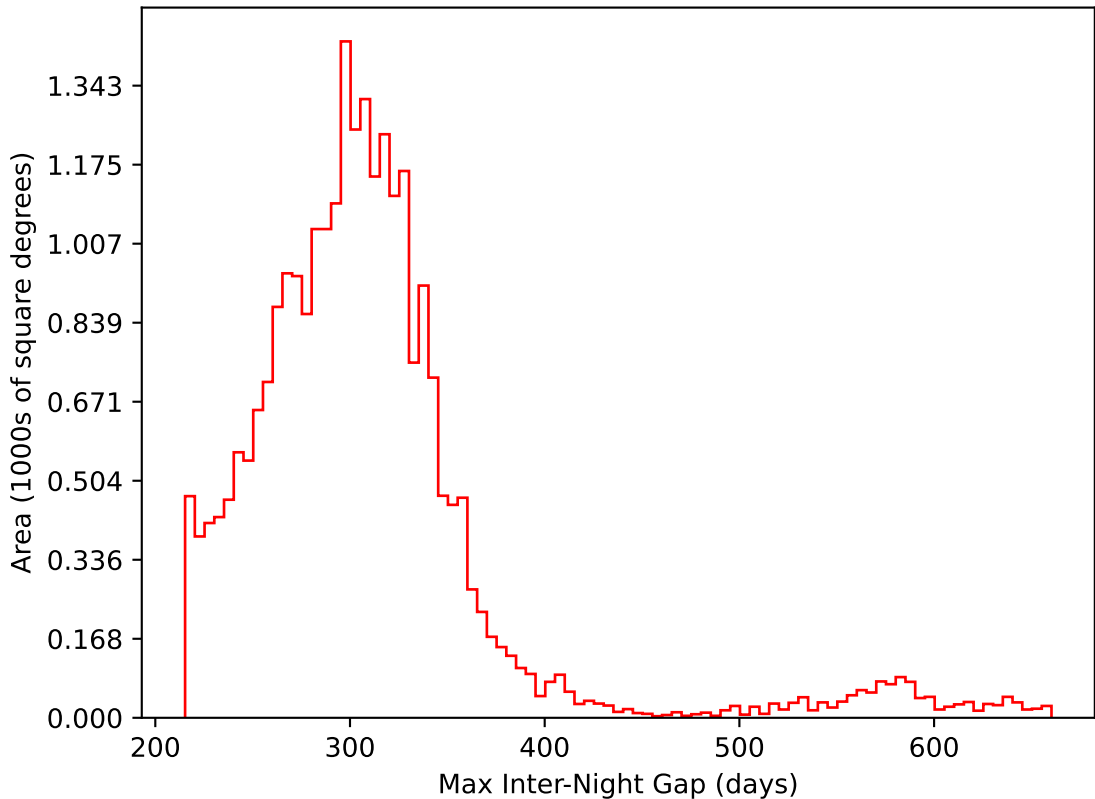
too_elab_r16_d2_giz_v3.4_10yrs All sky i band: Max Inter-Night Gap
